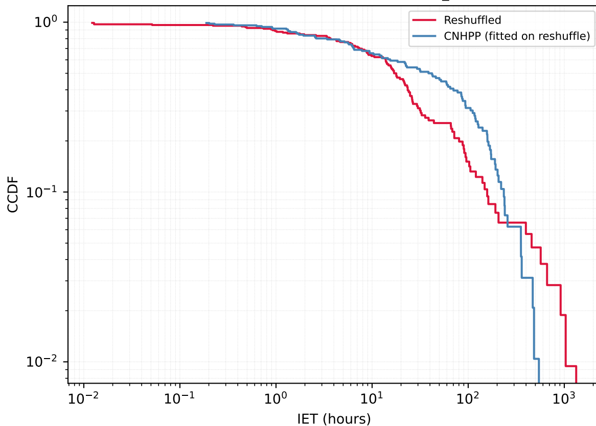
User 1134520908 - Reshuffled vs CNHPP A_{\text{fit}}=0.5295
